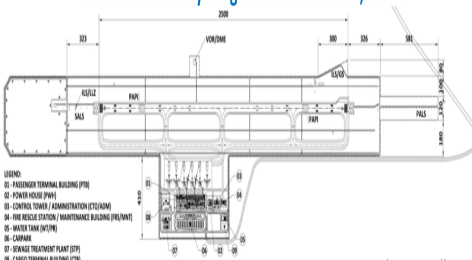
VO No.3A: Runway Length is extended to 2,500 m
